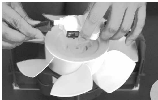
Fig 6. ... gently pull one of the motor assembly arm 1/8 inch ...
